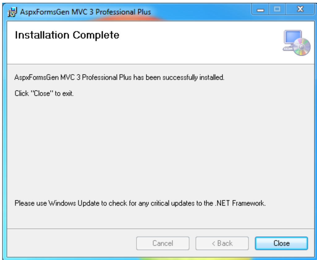
Figure 5 Installation Complete
