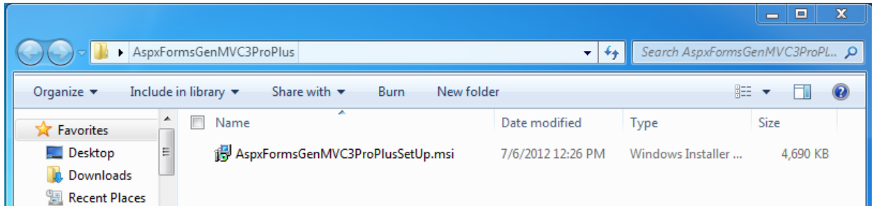
Figure 1 Unzipped Files
