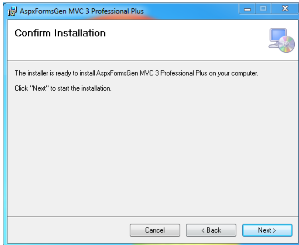
Figure 4 Confirm Installation
