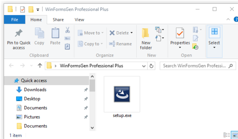
Figure 1 Unzipped Files
