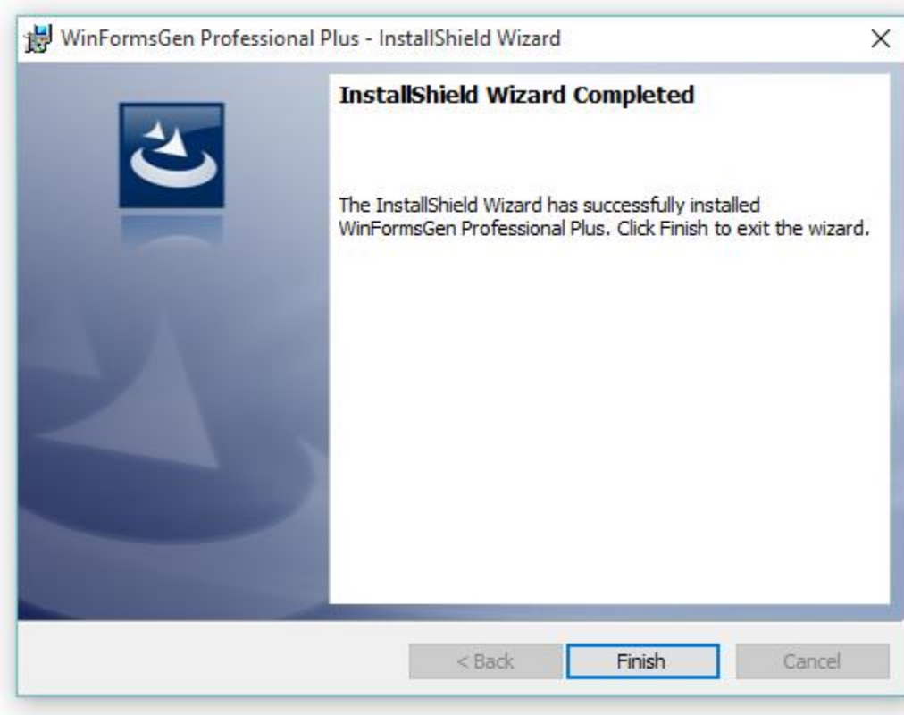
Figure 6 Installation Completed
